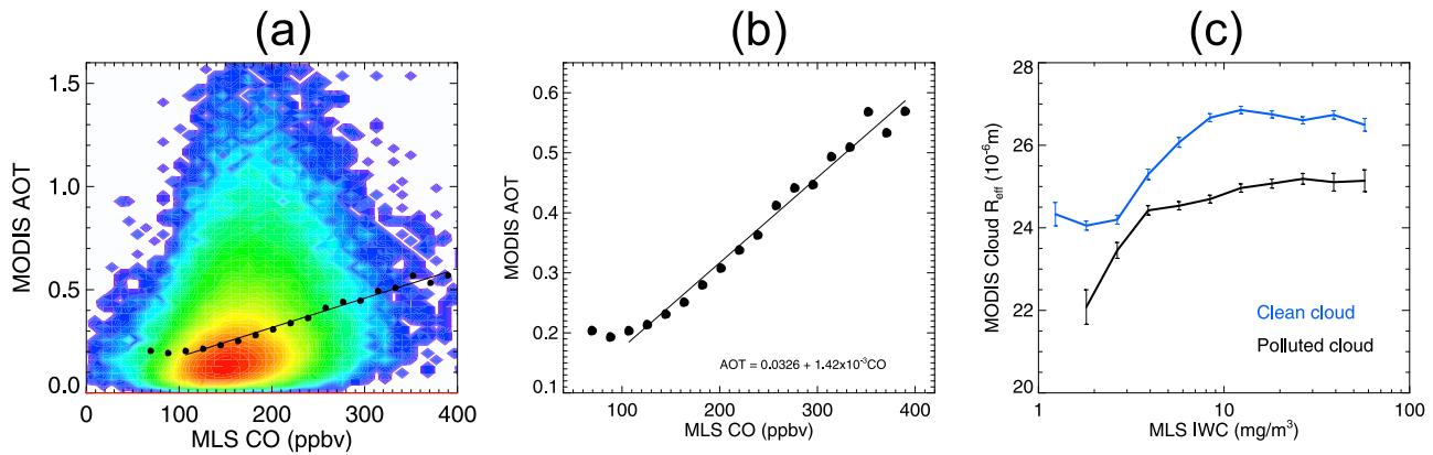
Figure 6. (a) The scatterplot of MODIS AOT versus MLS CO in cloudy regions ( IWC is \geq 2 \text{ mg/m}^3 ). The over-plotted black dots are the mean AOT data binned according to the collocated CO values, and the black-line is the linear fit to the binned AOT in the CO \geq 100 ppbv regions. (b) The black dots from Figure 6a are replotted for clarity. (c) MODIS r_e data binned according to the collocated MLS IWCs for clean ( CO \leq 100 ppbv) and polluted ( CO \geq 240 ppbv) clouds. All data from August 2004 to July 2008 between 50^\circ S and 50^\circ N are used for this plot.
